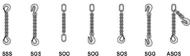
SINGLE LEG CHAIN SLING STYLES
